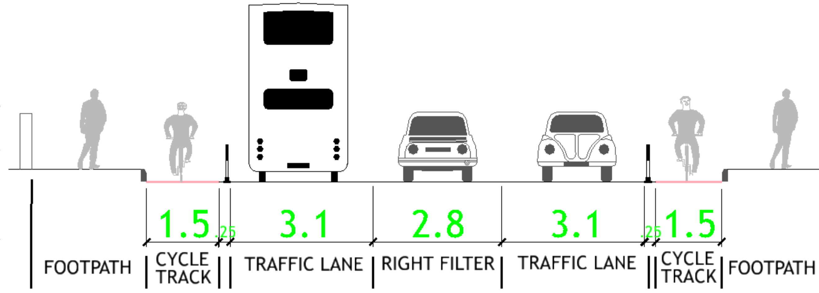
SECTION DETAIL: b - b
